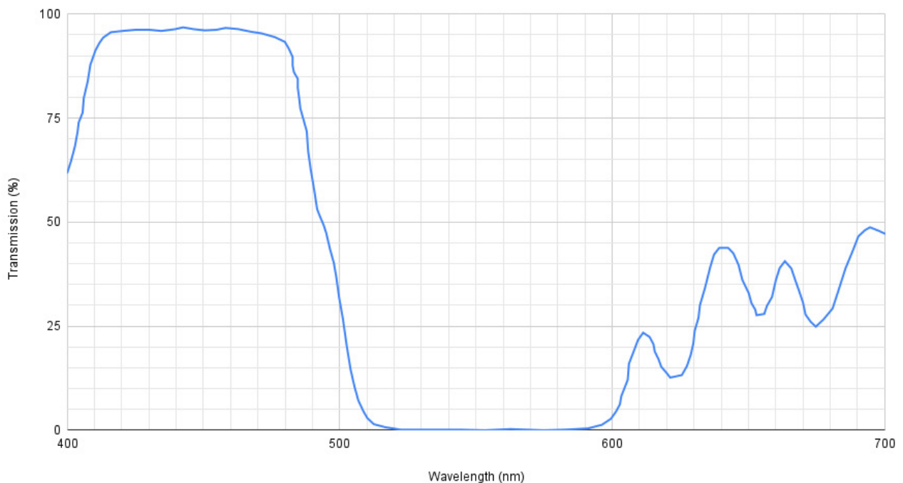
Dichroic Filter "refl. green pass blue"
