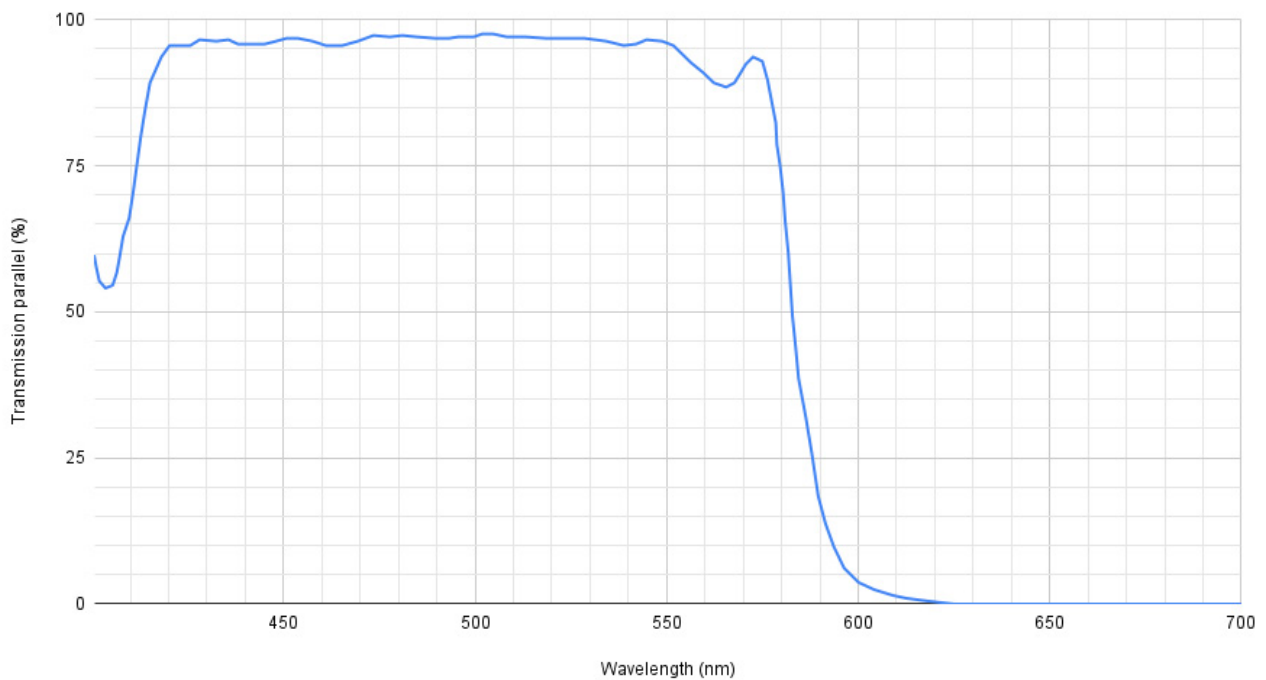
Dichroic Filter "refl. red" (parallel, p)
