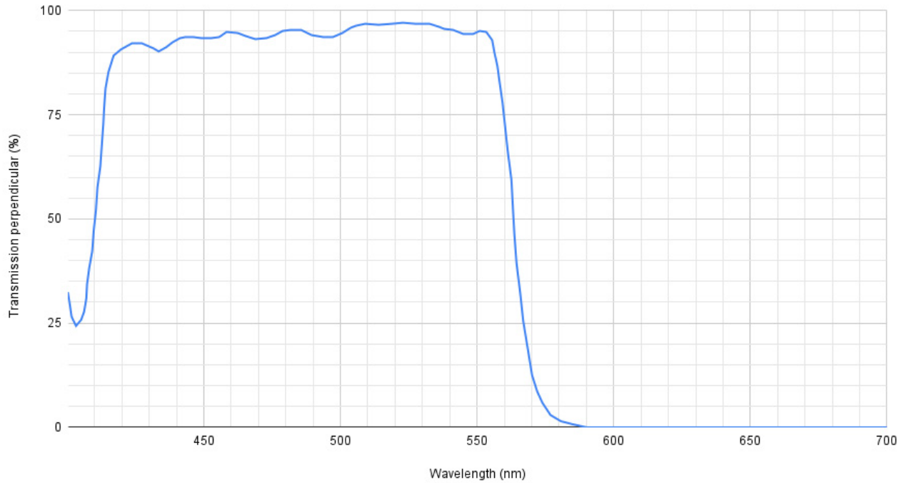
Dichroic Filter "refl. red" (perpendicular, s)
